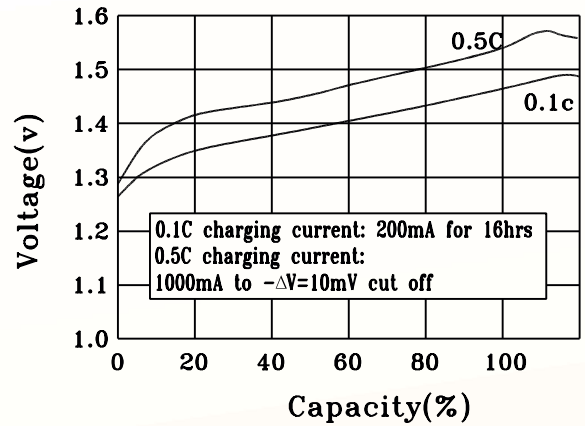
CHARGE CHARACTERISTICS
