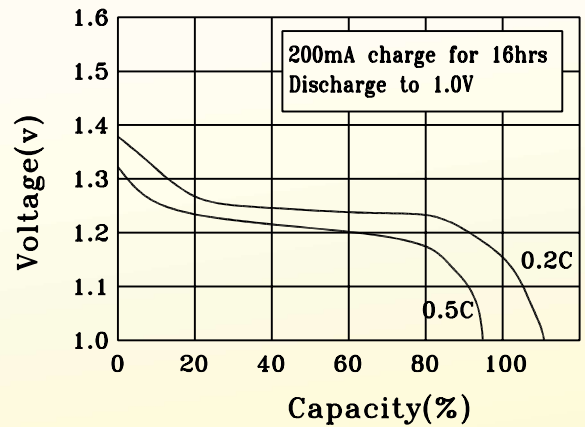
DISCHARGE CHARACTERISTICS
